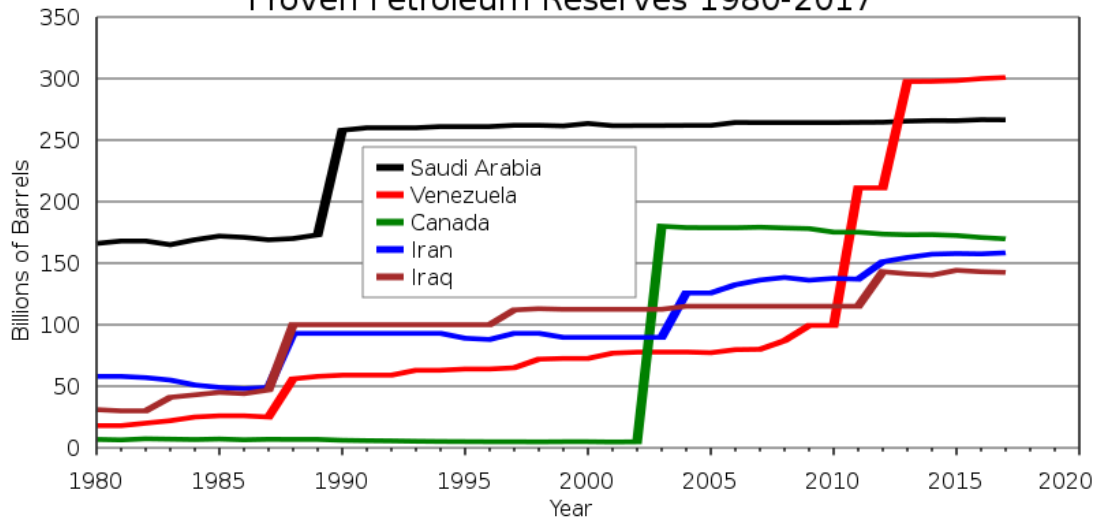
Proven Petroleum Reserves 1980-2017
